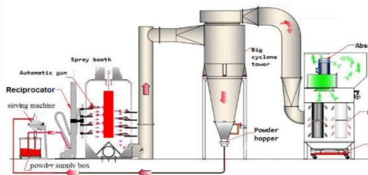
Powder spray booth system -Big cyclone serie
